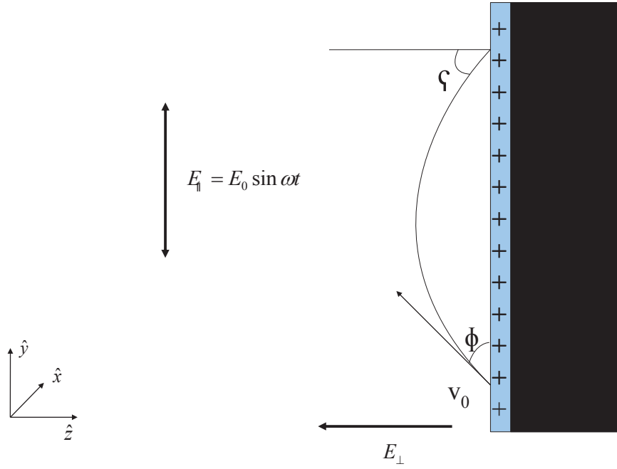
Figure 4. Trajectory of the secondary electron. v_0 is the electrons initial energy, \phi is the electron's initial emission angle, and \varsigma is the angle at which the particle impacts the dielectric surface.
